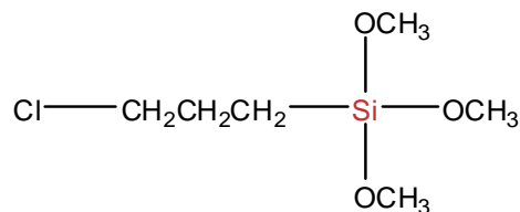
3-trimethoxysilyl-1-chloropropane
